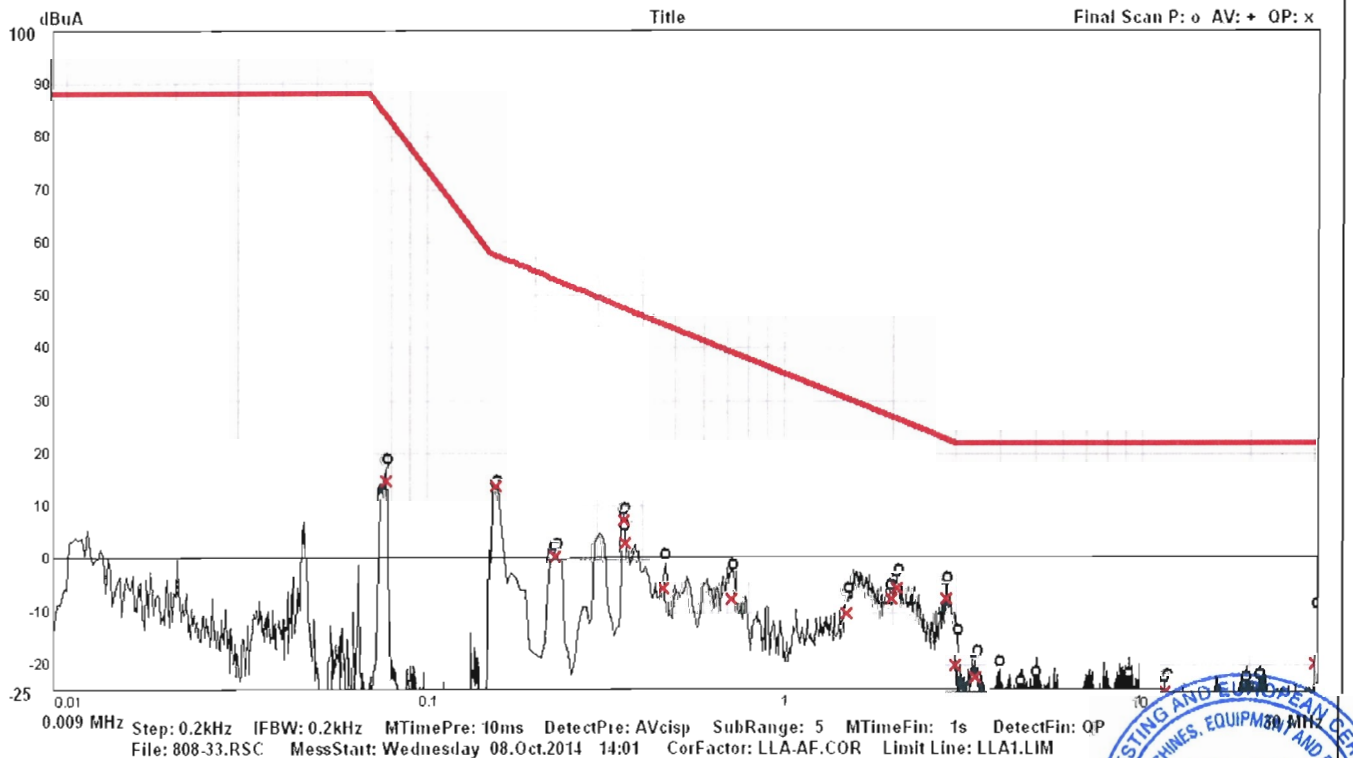
Drawing of Radiated electromagnetic disturbances - measured along the axis - Z
